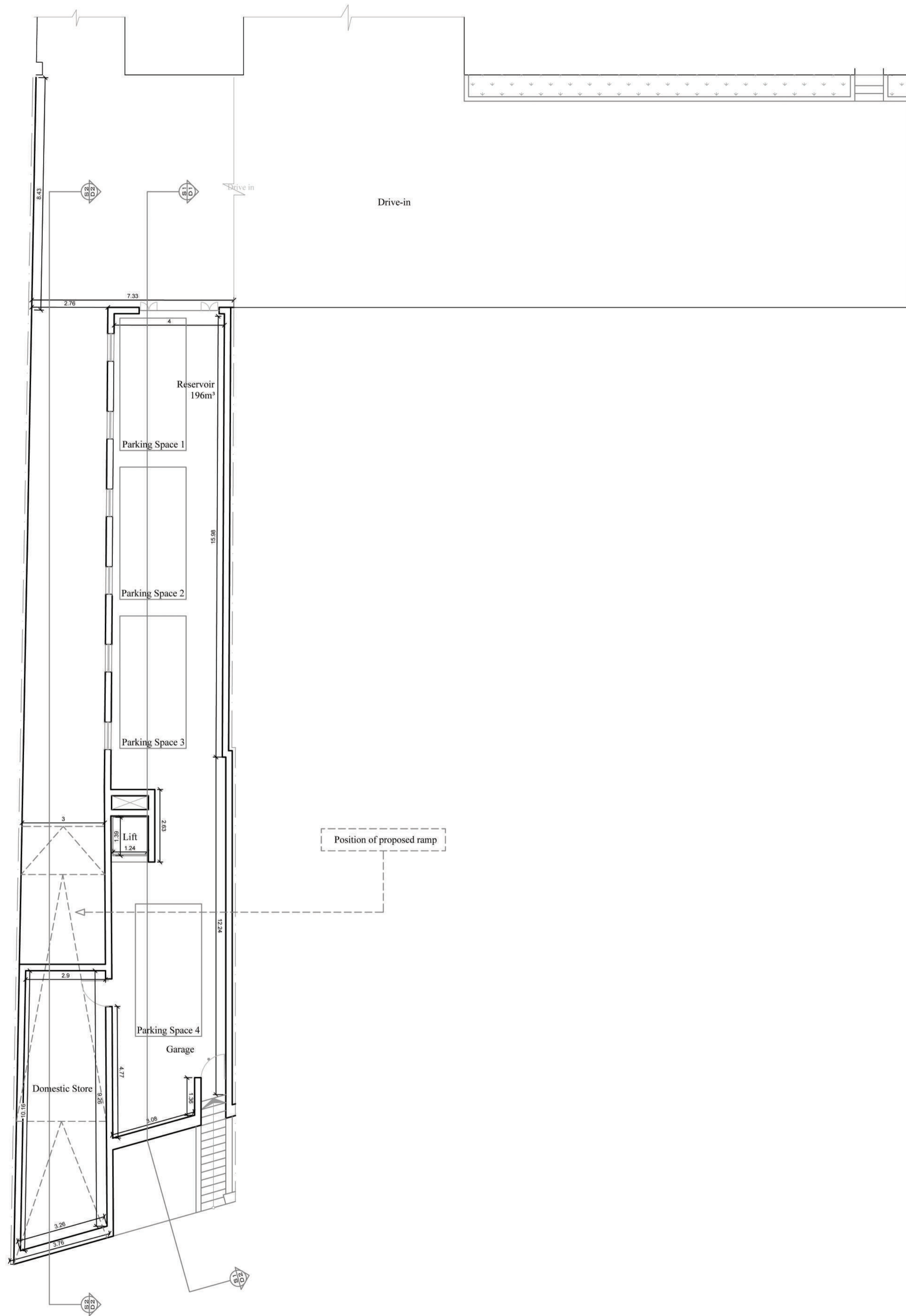
P1 D3 Approved and Proposed Basement Level (No Changes) Scale 1:100
