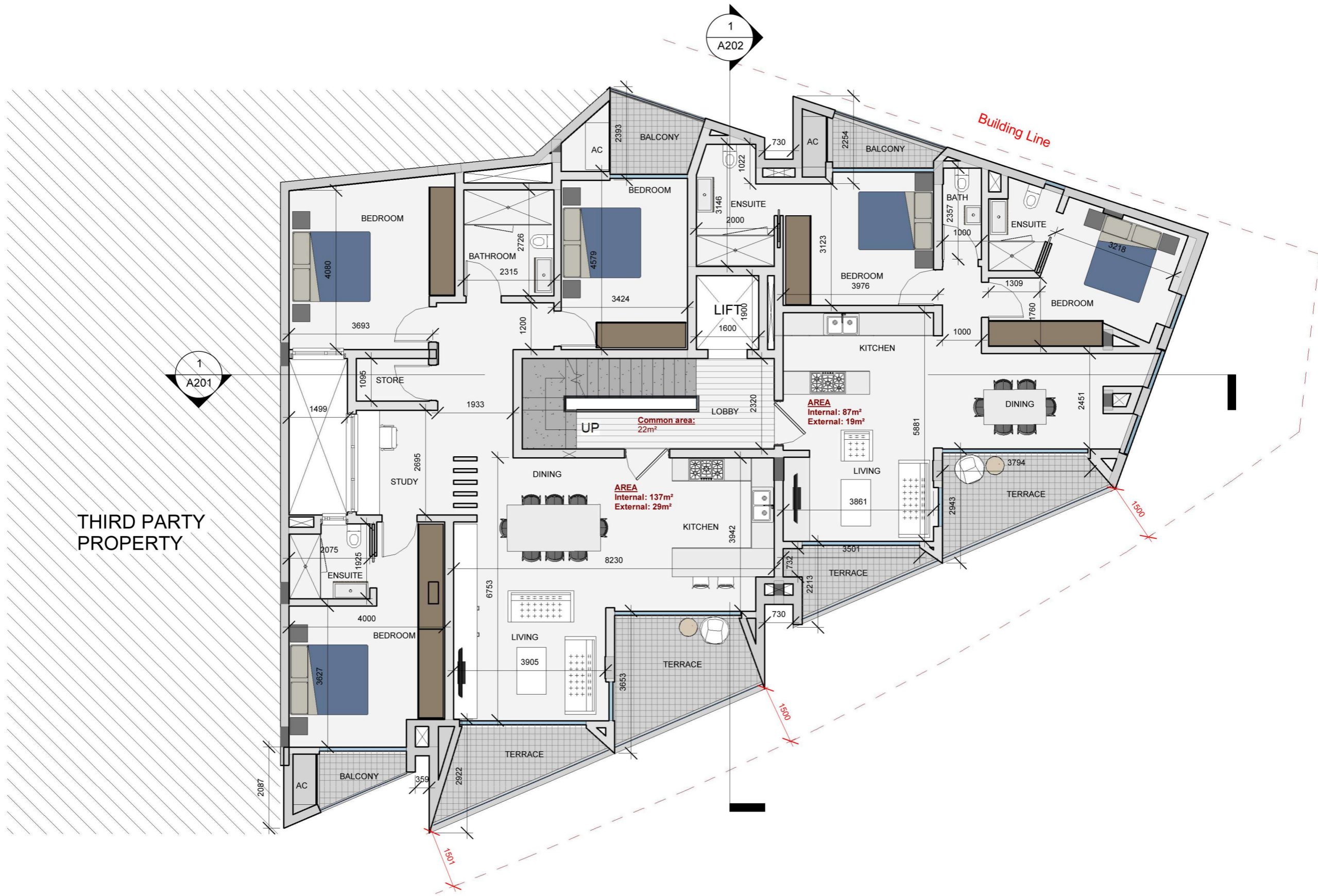
1 Proposed Level 2 1 : 100
