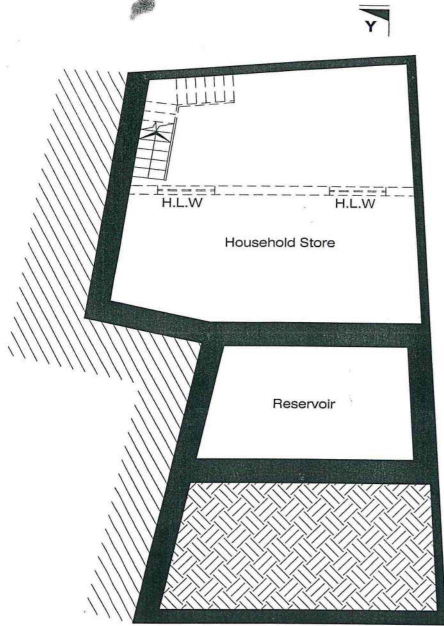
Proposed Basement Floor Plan Scale 1:100
