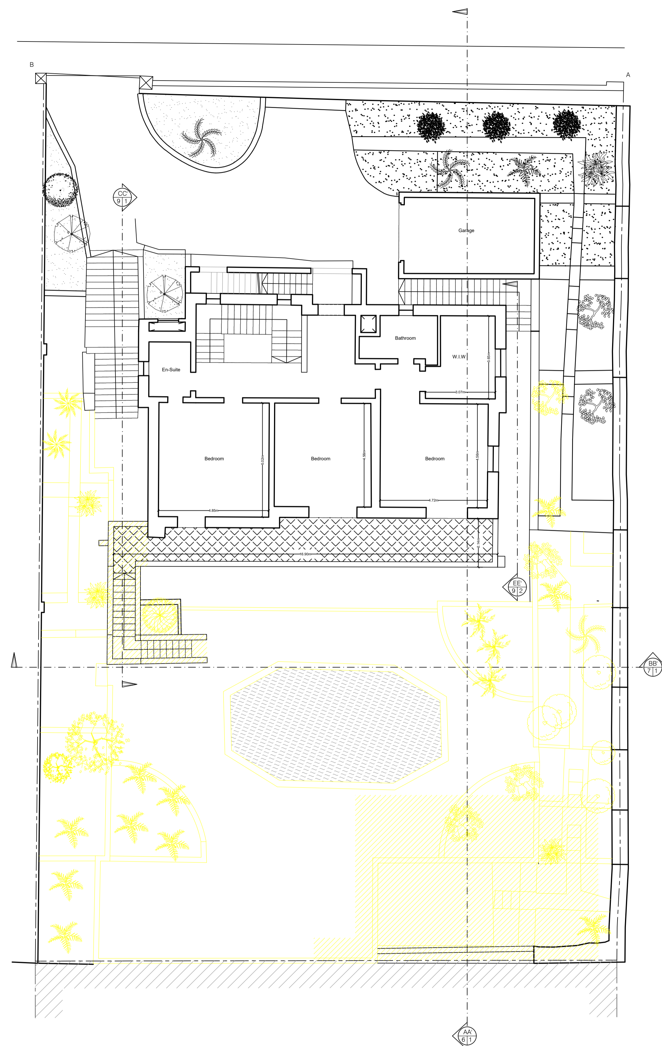
② Existing Ground Floor Scale 1:100
