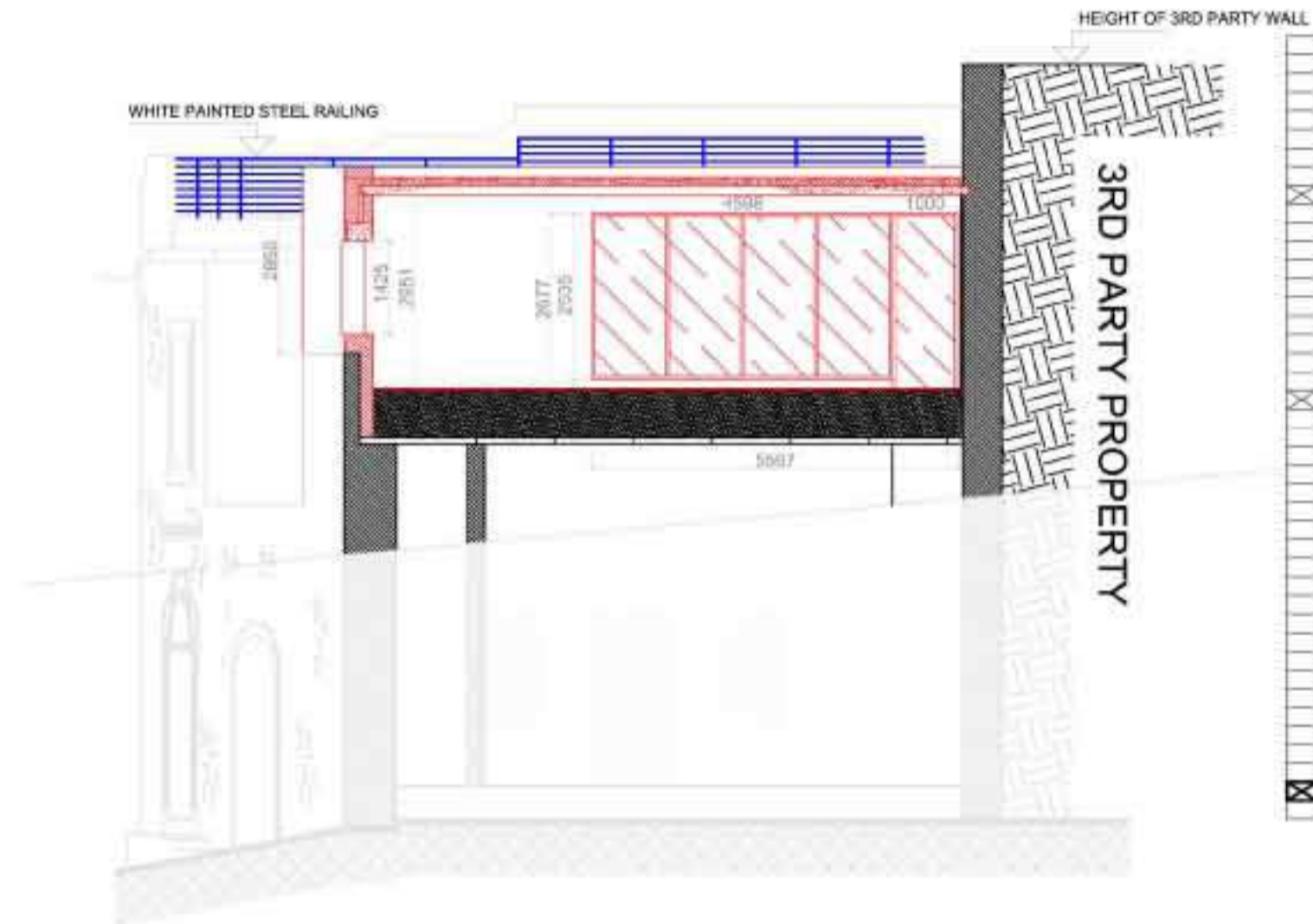
15 PROPOSED SECTIONAL ELEVATION EE' Scale 1:100
