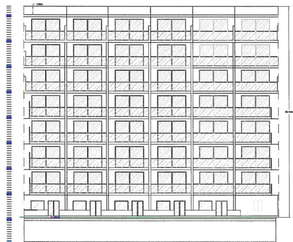
PROPOSED ELEVATION - scale 1:100
