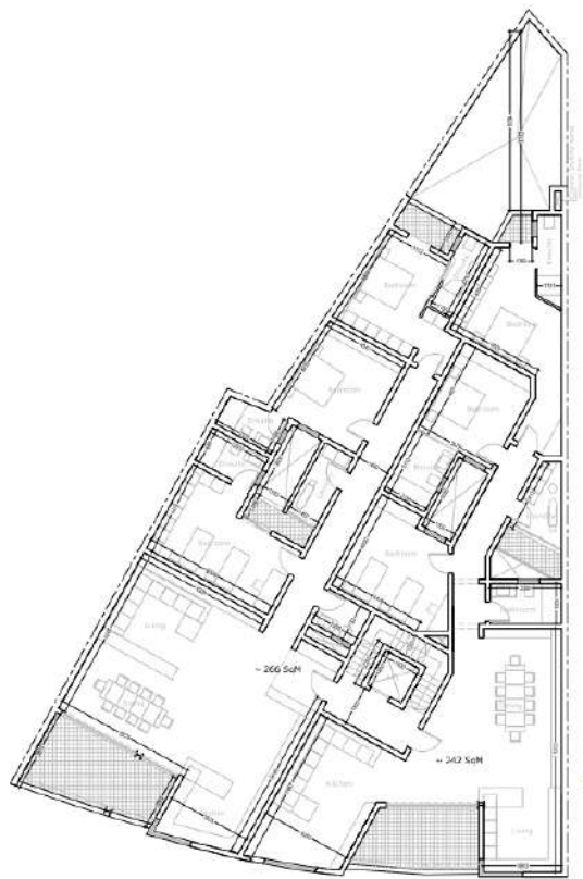
First Floor Level As Approved in PA/11055/18
