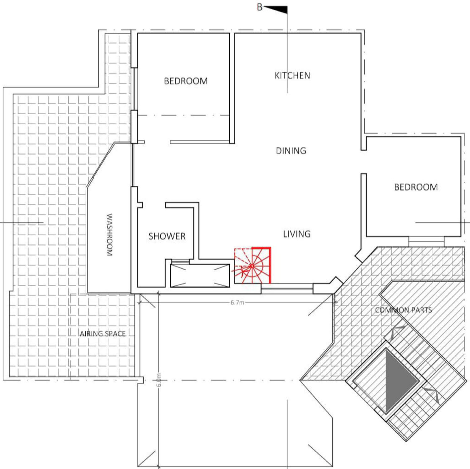
EXISTING / PROPOSED FOURTH FLOOR LEVEL SCALE 1:100
