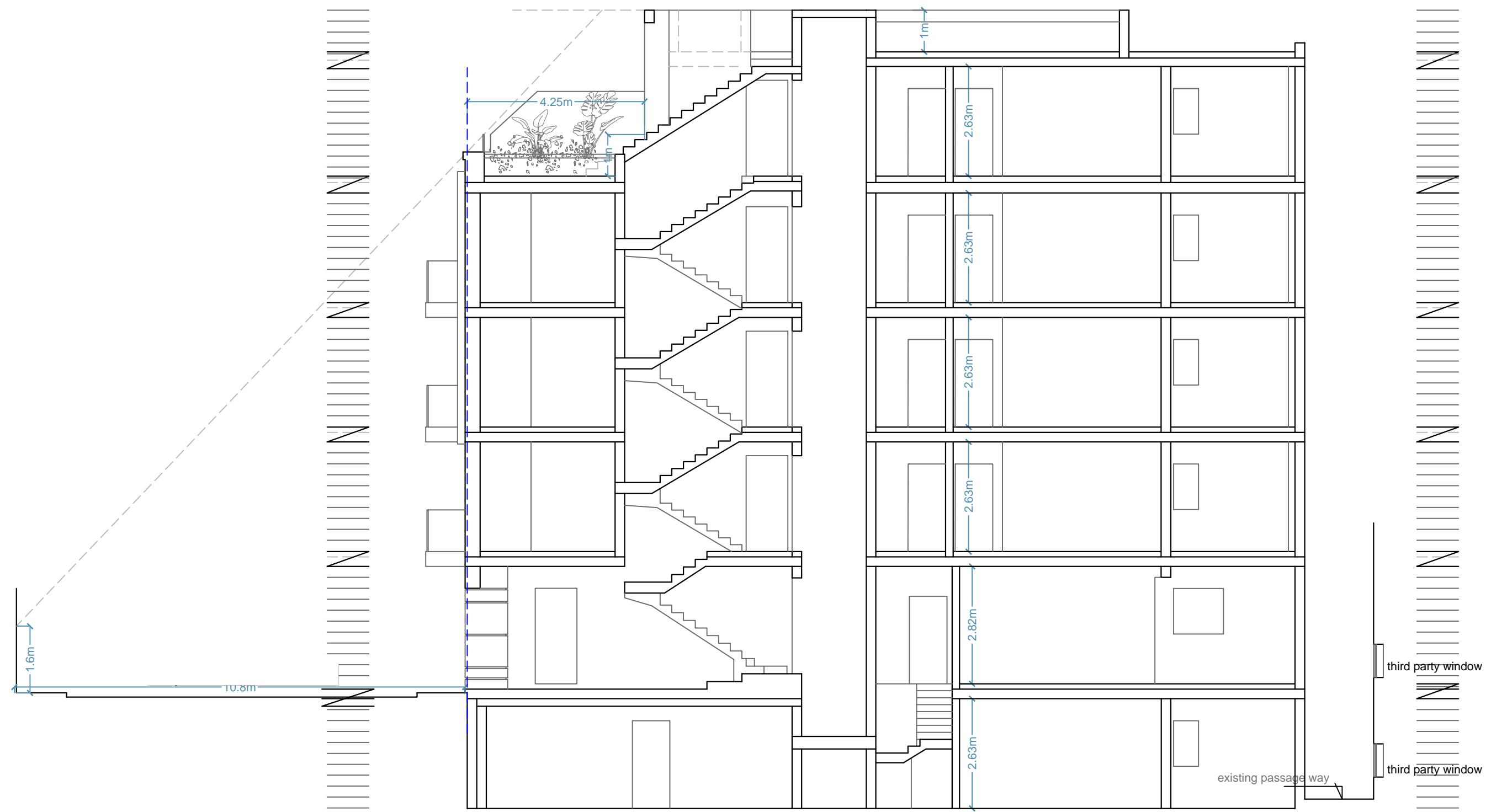
Section B-B
