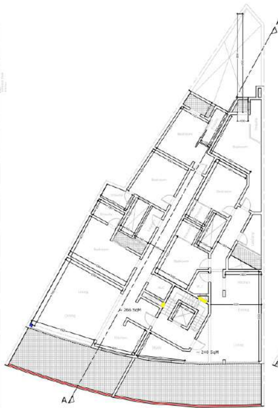
Fourth Floor Level Plan Proposed Changes Colour Coded
