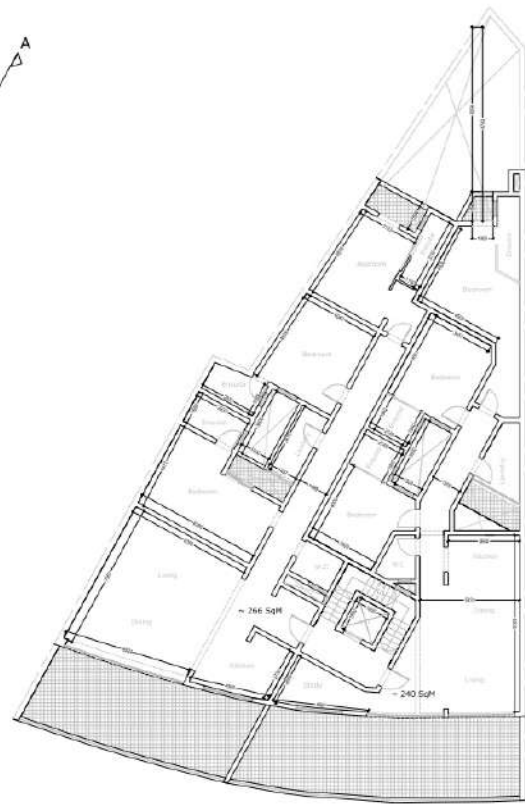
Proposed Fourth Floor Level Plan
