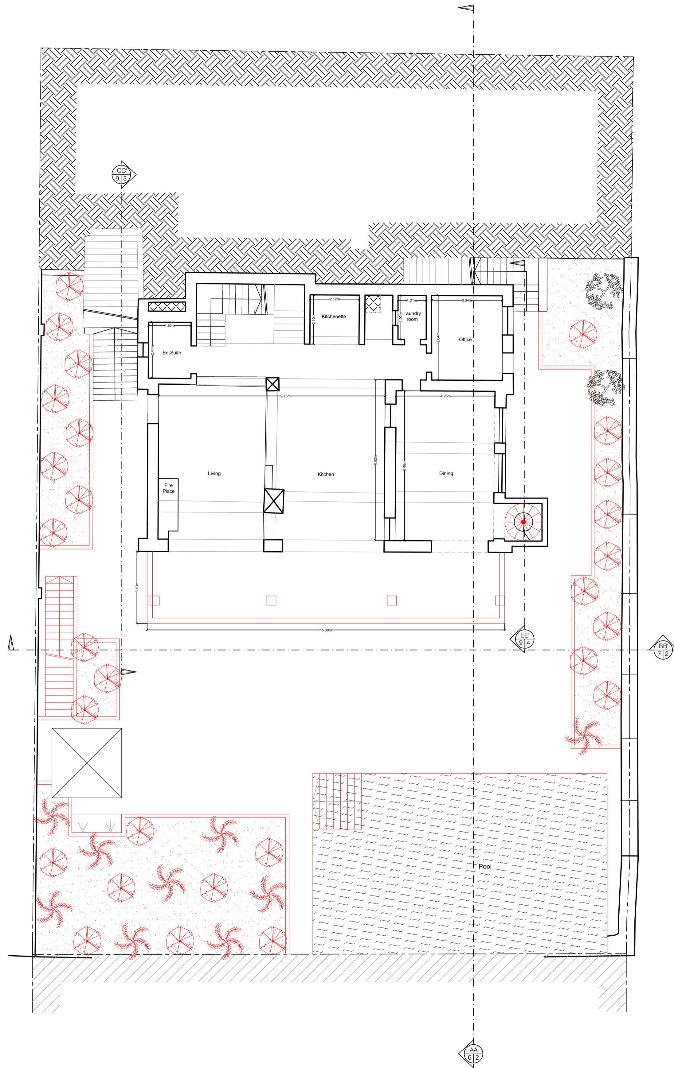
① Proposed Basement (-1) Floor Scale 1:100
