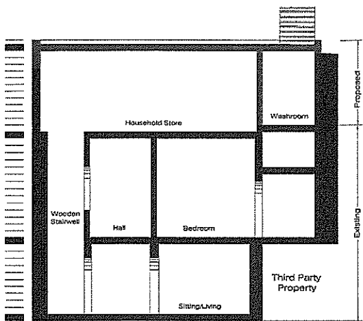
Existing/Proposed Section A-A Scale 1:100
