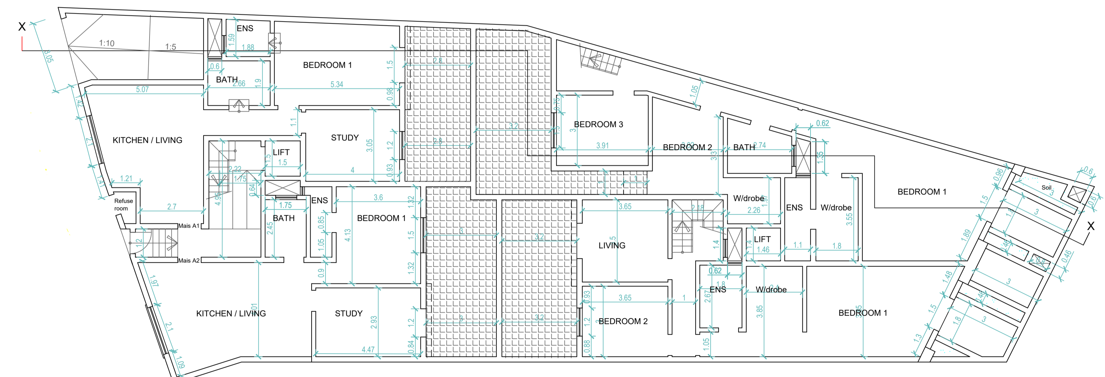
LEVEL 0
